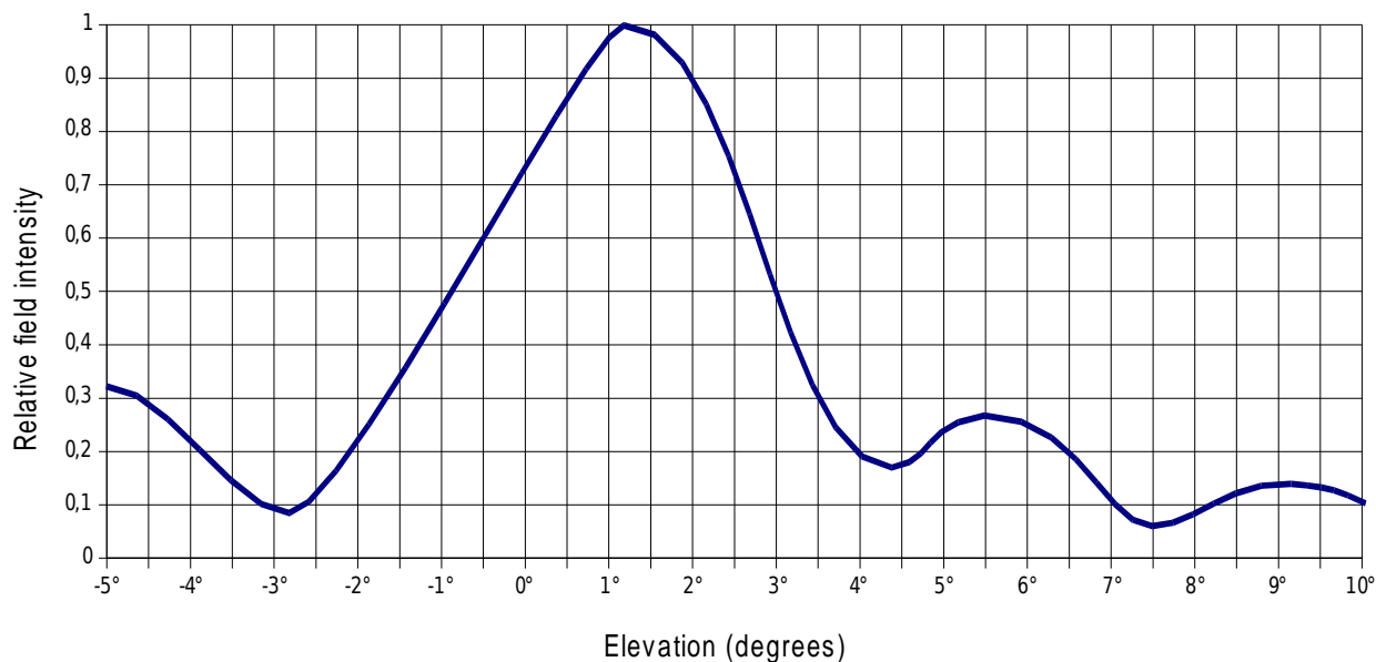
Antenna for MMDS - 15 dBi
