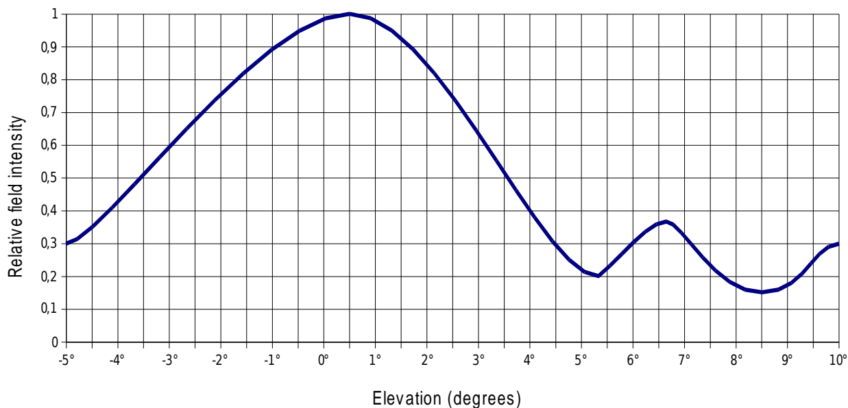
Antenna for MMDS - 11 dBi
