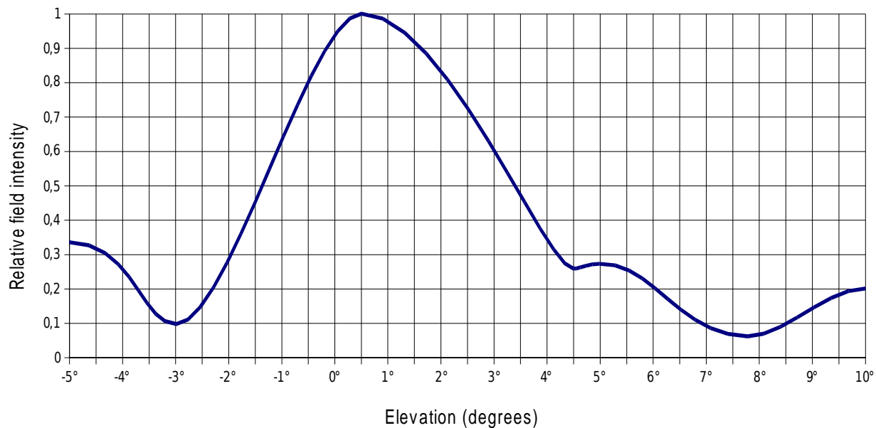
Antenna for MMDS - 16 dBi
