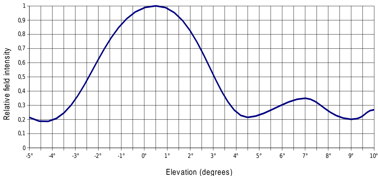
Antenna for MMDS - 13 dBi
