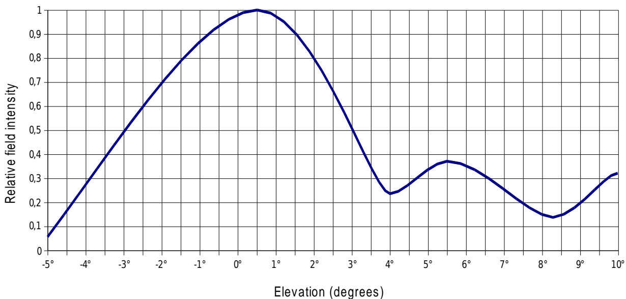
Antenna for MMDS - 14 dBi
