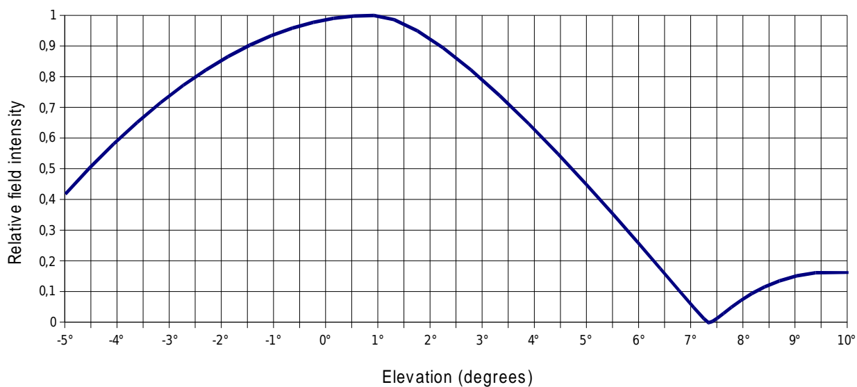
Antenna for MMDS - 8 dBi
