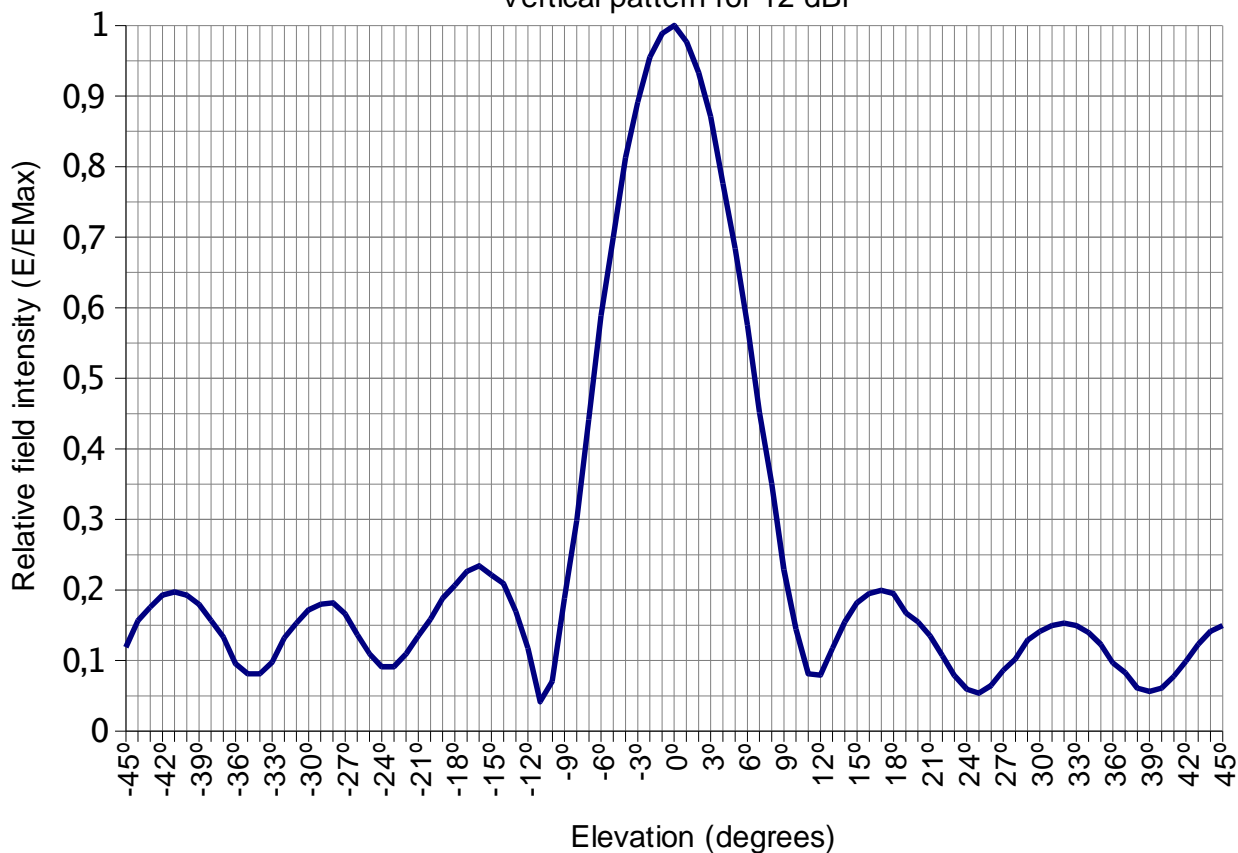
Sectorial Panel for WLL Vertical pattern for 12 dBi
