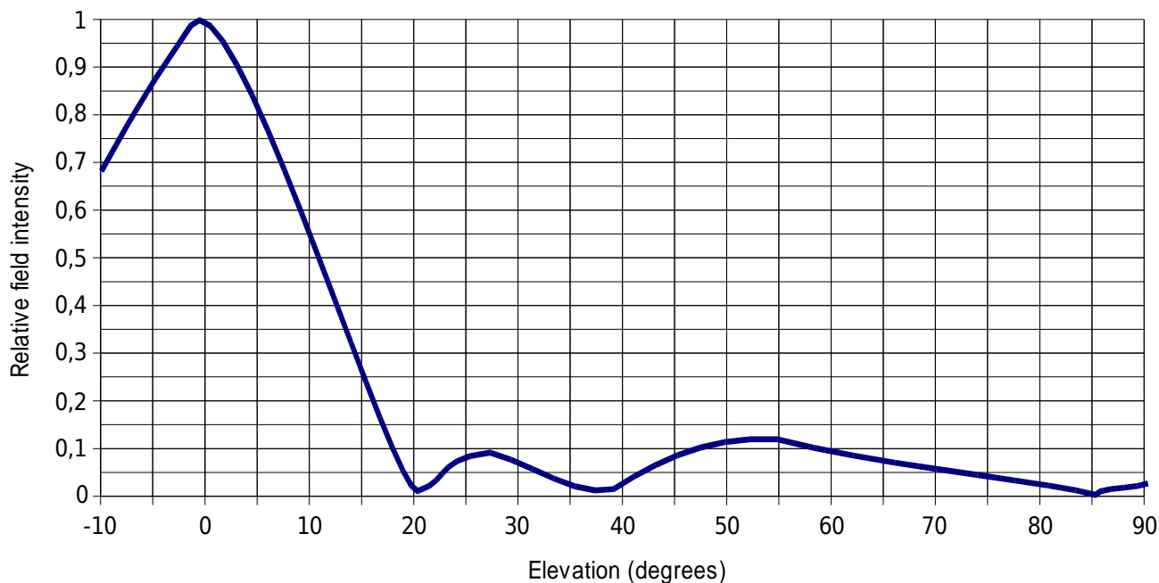
Half wave dipoles Panel – UHF 6 bays vertical pattern – Half power angle: 16°
