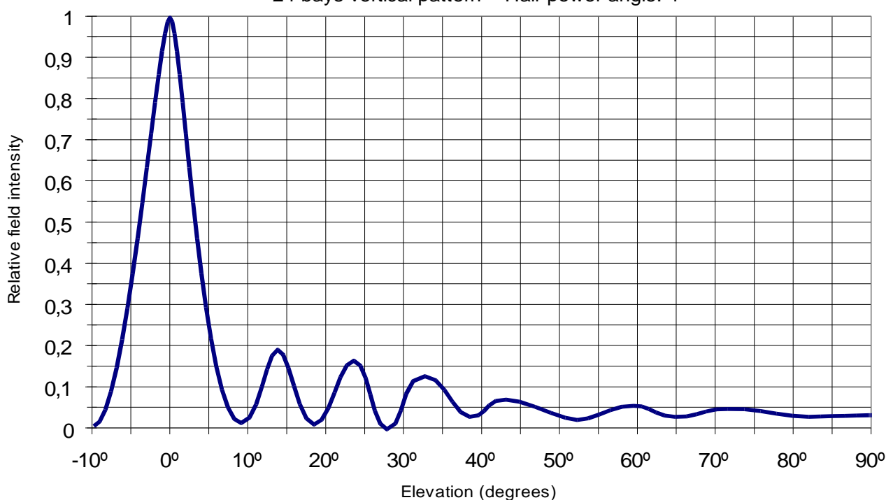
Half wave dipoles Panel – UHF 24 bays vertical pattern – Half power angle: 4°
