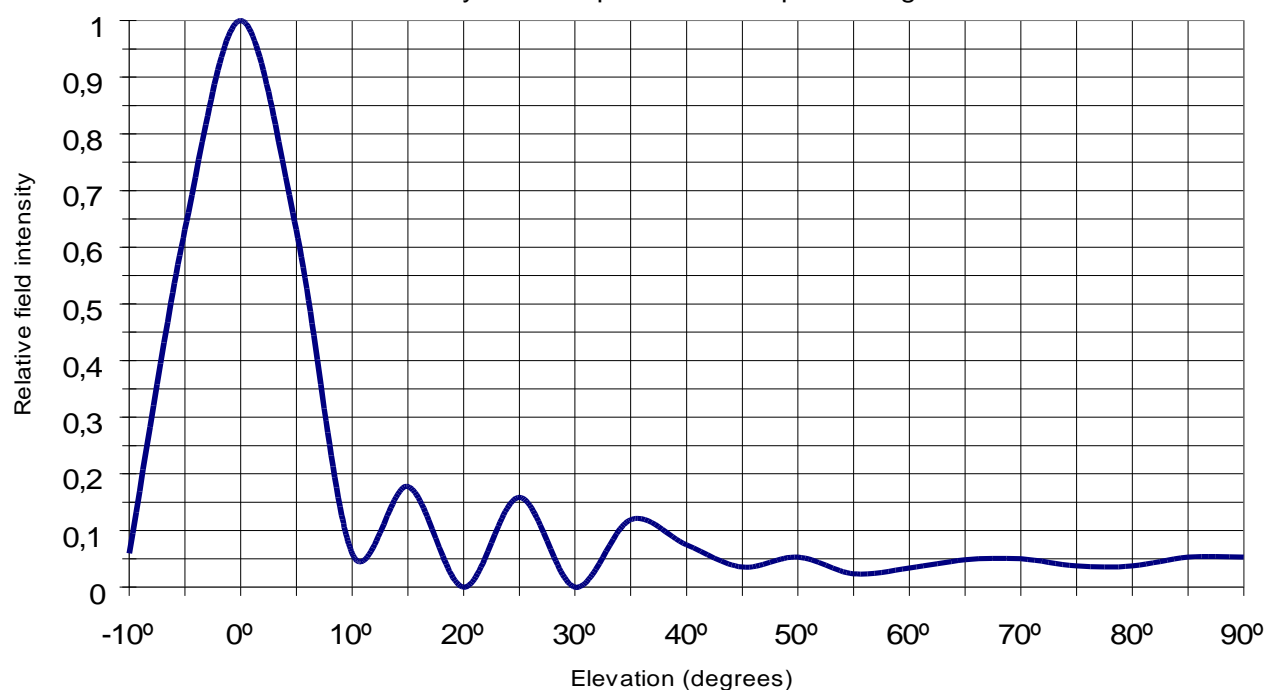
Half wave dipoles Panel – UHF 12 bays vertical pattern – Half power angle: 8°
