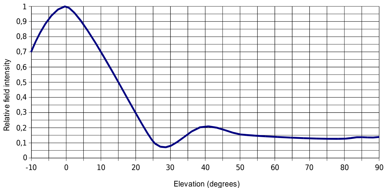
Half wave dipoles Panel – UHF 4 bays vertical pattern – Half power angle: 24°
