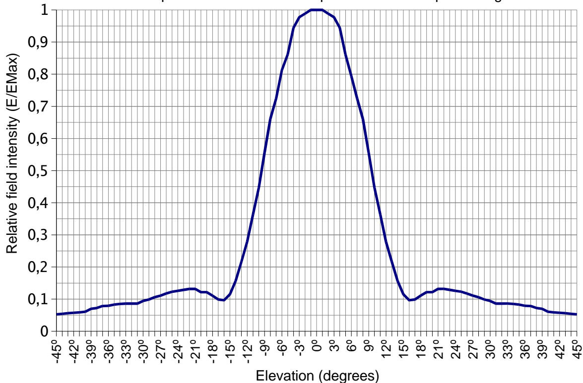
Parabolic Antenna with reflector size of 2m - UHF Horizontal pattern for the horizontal polarization - Half power angle: 14°
