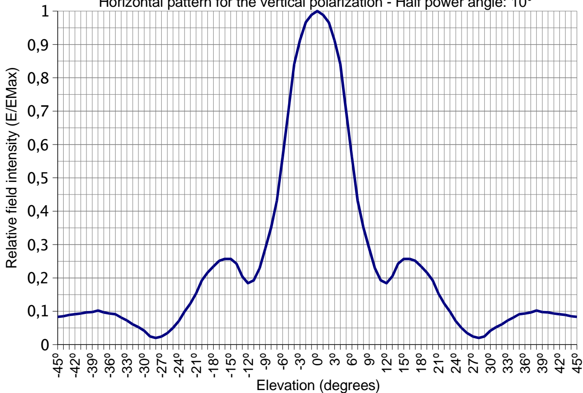
Parabolic Antenna with reflector size of 2m - UHF Horizontal pattern for the vertical polarization - Half power angle: 10°
