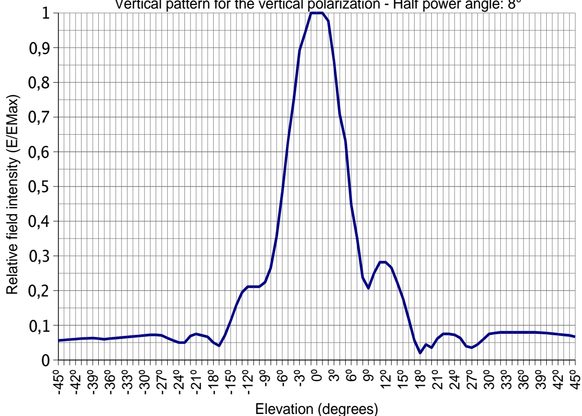
Parabolic Antenna with reflector size of 3m - UHF Vertical pattern for the vertical polarization - Half power angle: 8°
