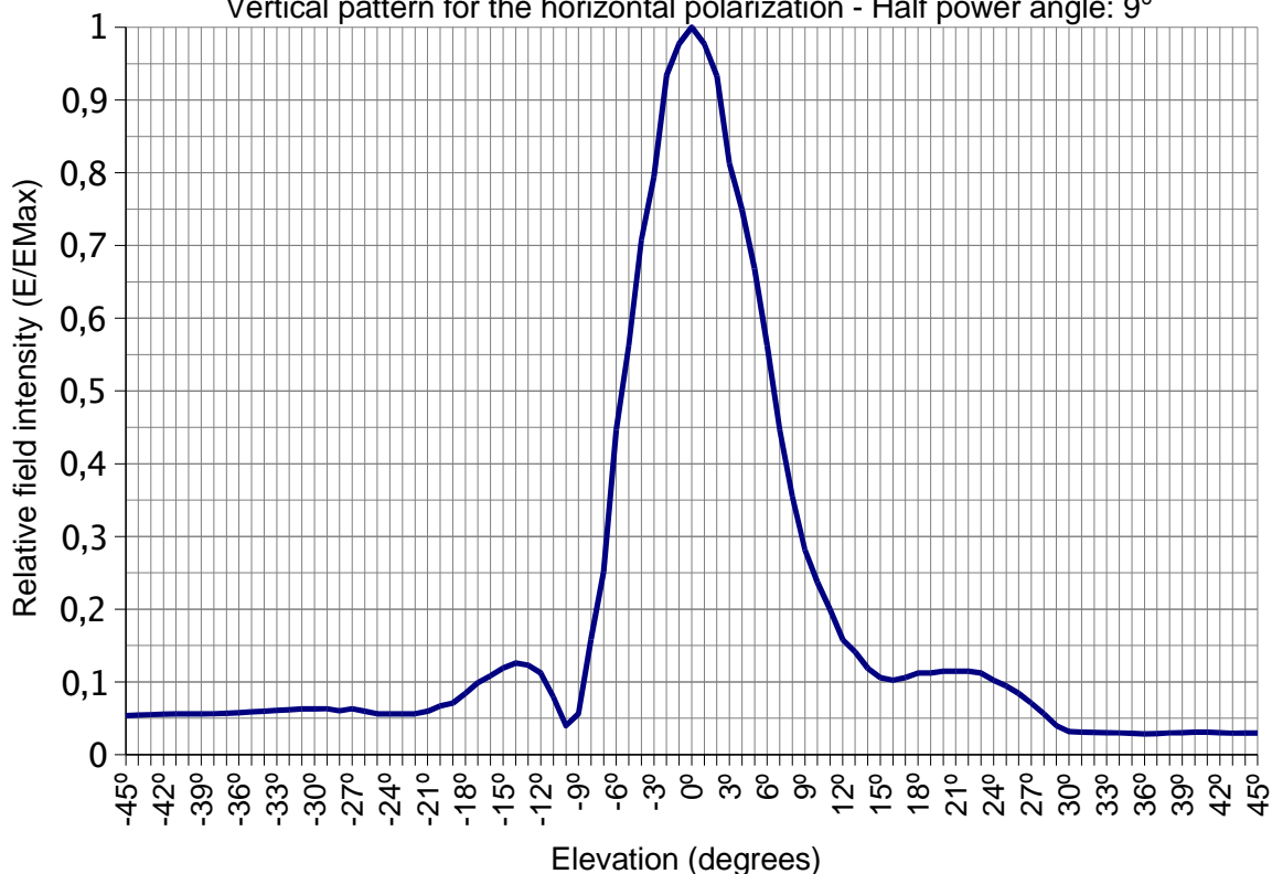
Parabolic Antenna with reflector size of 3m - UHF Vertical pattern for the horizontal polarization - Half power angle: 9°
